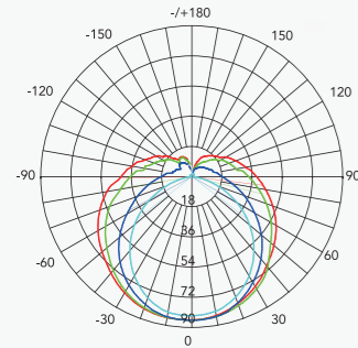
Illuminance Distribution
