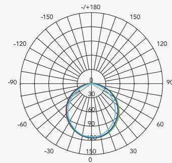
Illuminance Distribution
